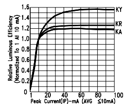
Fig5. RELATIVE LUMINOUS EFFICIENCY (LUMINOUS INTENSITY PER UNIT CURRENT) VS. PEAK CURRENT
